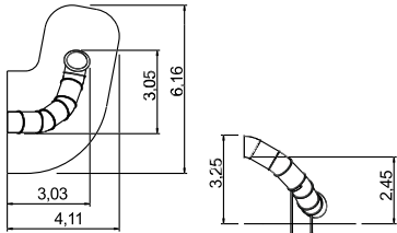
Spiral slide 120 degrees spiral left PH 245 cm
