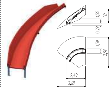
Hill slide curved left
