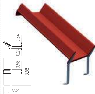
Hill slide straight 100cm
