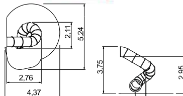
Spiral slide 270 degrees spiral left PH 295 cm
