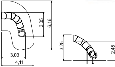
Spiral slide 120 degrees spiral right PH 245 cm
