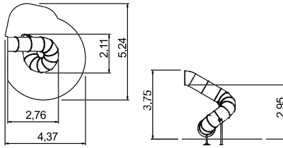
Spiral slide 270 degrees spiral right PH 295 cm
