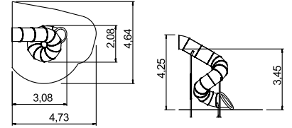
Spiral slide 360 degrees spiral right PH 345 cm
