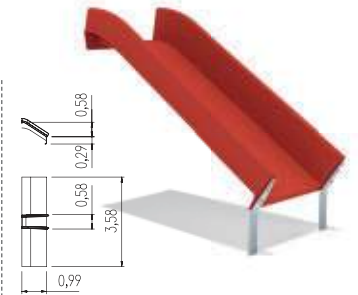
Hill slide entry plate
