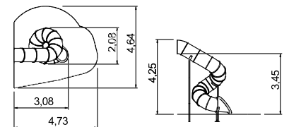
Spiral slide 360 degrees spiral left PH 345 cm
