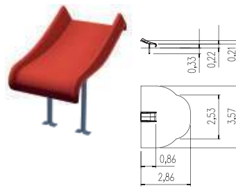
Hill slide short end
