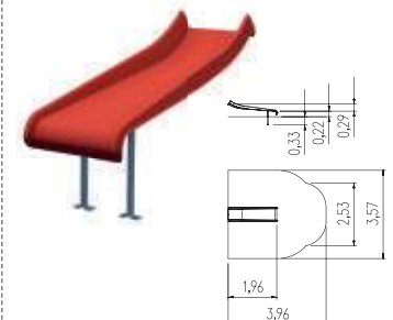
Hill slide long end
