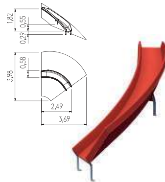
Hill slide curved right
